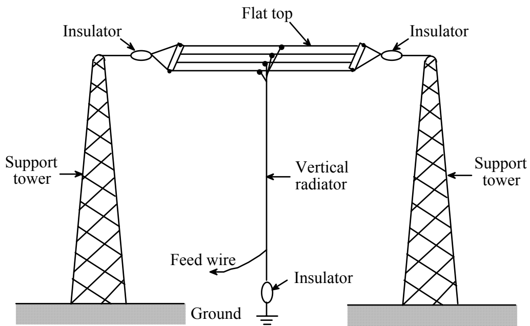
Fig. 4. A top-loaded short-monopole antenna typical of VLF/LF communication systems.
