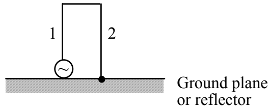
(a) A folded monopole antenna
