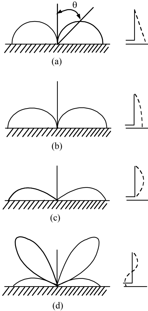
Fig. 3. Radiation patterns for some typical end-fed vertical monopoles above infinite ground: (a) h/\lambda = 0.05 (short monopole), (b) h/\lambda = 0.15 (quarter-wave monopole), (c) h/\lambda = 0.5 (half-wave monopole), and (d) h/\lambda = 0.75 ( 3/4 \lambda monopole) [adapted from E. C. Jordan and K. G. Balmain (1)].
