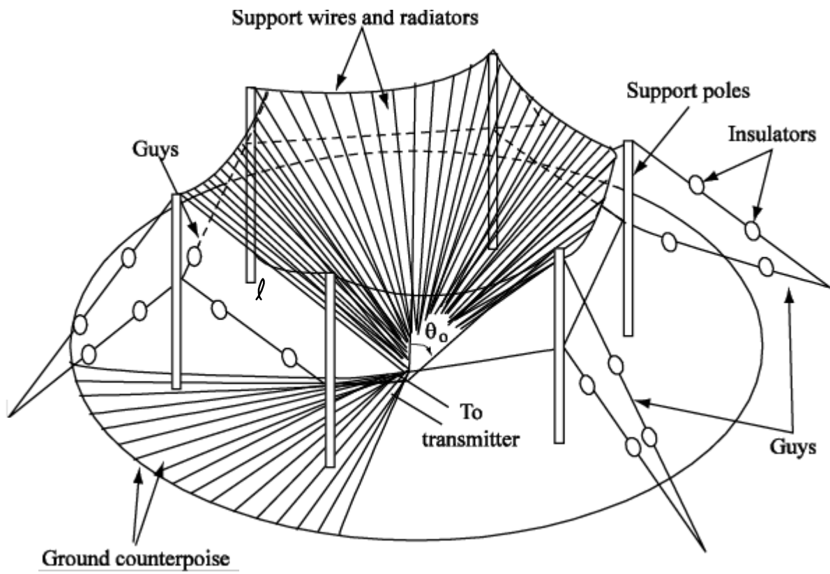
Fig. 7. A conical monopole.
