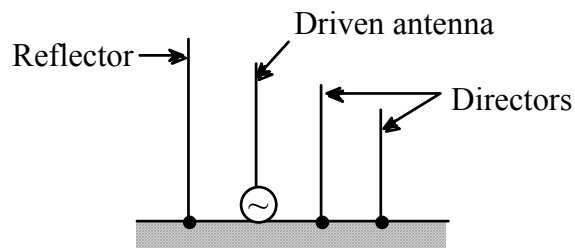
(c) A 4-element Yagi-Uda array of monopoles
