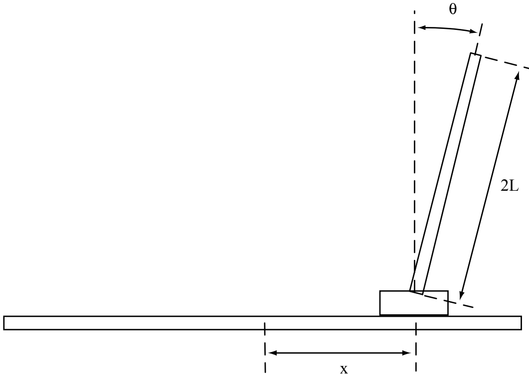
Figure 8.32: Inverted Pendulum System
